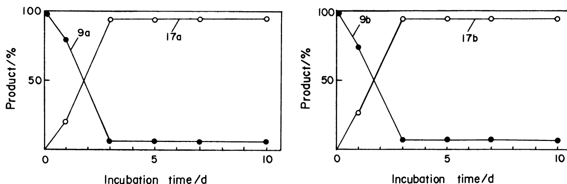
Fig. 4. The time-courses in the biotransformation of the enantiomeric pairs of neoisooverbanols ( 9a and 9b ).
